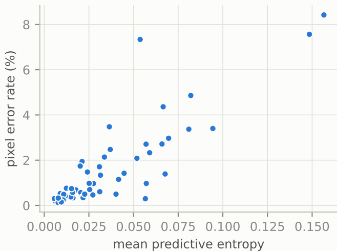
Per-image: entropy vs error ( r = 0.86 )
